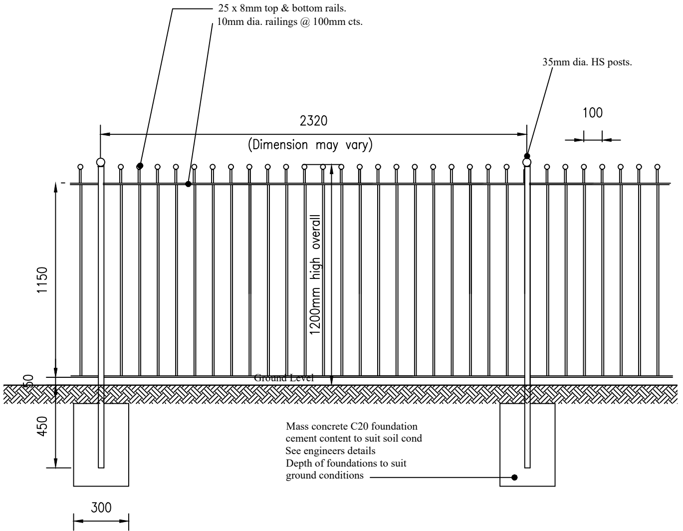
Front Elevation
