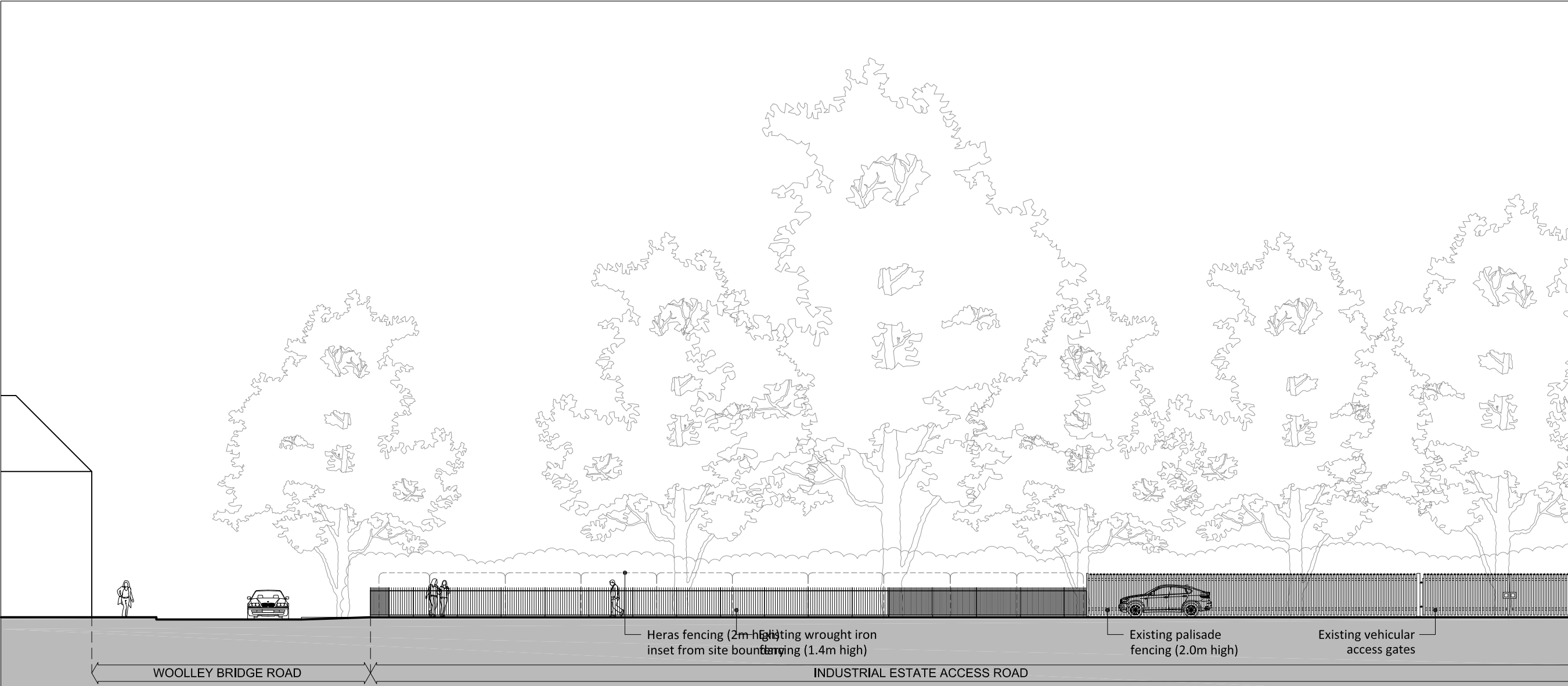
Existing elevation (B-B) to Etherow Industrial Estate access road
