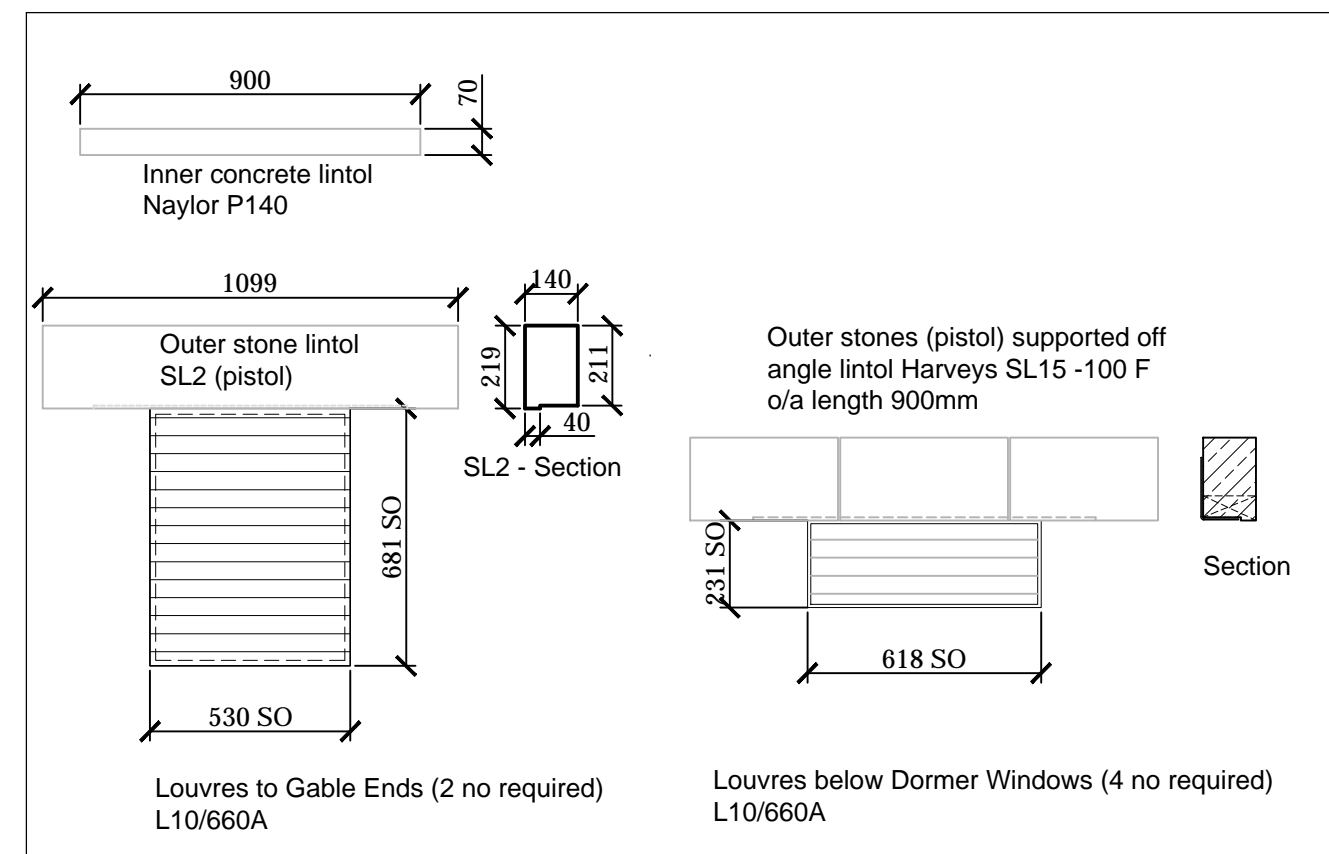
EXTERNAL LOUVRES (1:20)
