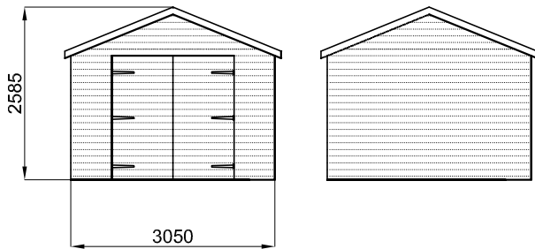
Storage Shed Elevations
