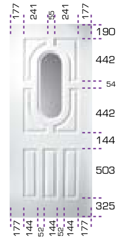
ARCACIA GLAZED Sash size. MAX 888 x 2098 MIN 726 x 1745 Frame size with Threshold. HxW. MAX 1000 x 2176 MIN 838 x 1823
