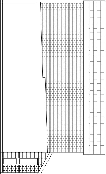
Proposed Side (North) Elevation 1:100 Unchanged
