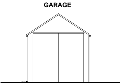
ELEVATION A 1:100
