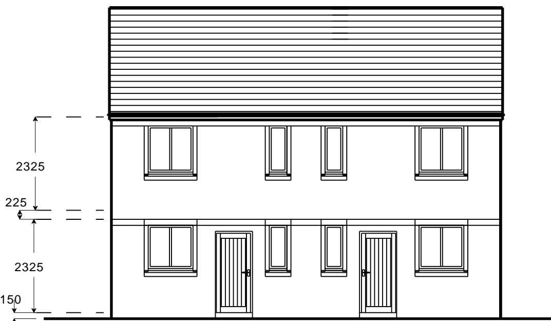
FRONT ELEVATION
