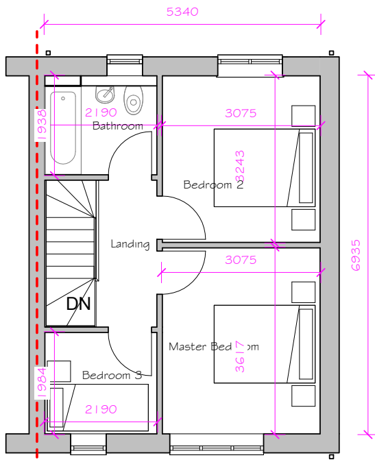
FIRST FLOOR PLAN OVERVIEW 1 : 100
