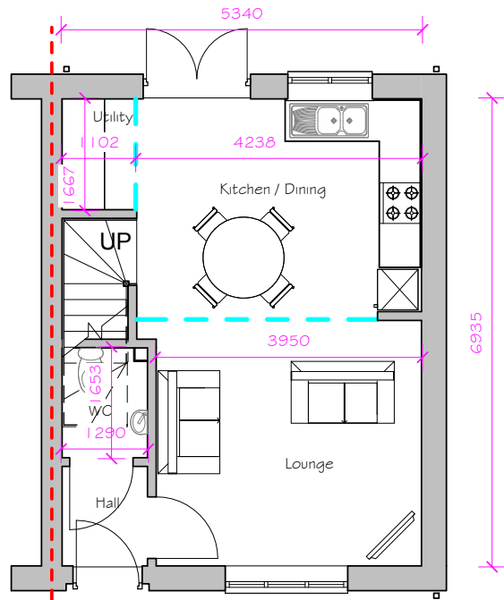
GROUND FLOOR PLAN OVERVIEW 1 : 100
