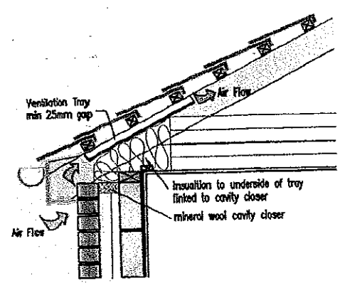
EAVES DETAIL
