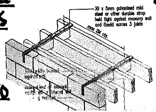
EAVES DETAIL
