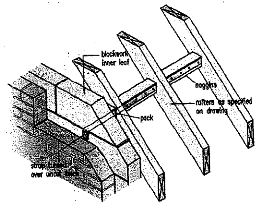
EFFECTIVE STRAPPING AT GABLE WALL
