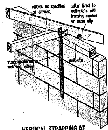
VERTICAL STRAPPING AT EAVES OF PITCHED ROOFS
