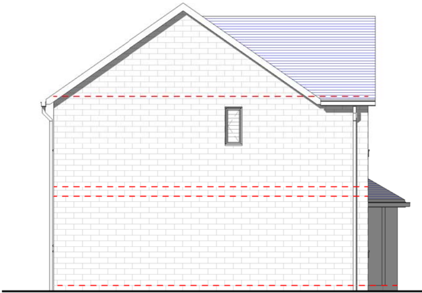
LEFT SIDE ELEVATION OVERVIEW 1 : 100
