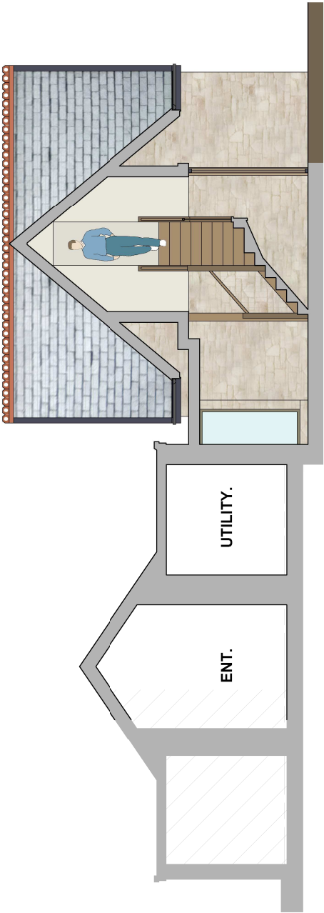
Section A (New roof - cross section)
