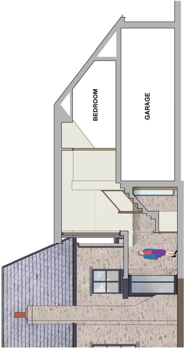
Section C (Garage)
