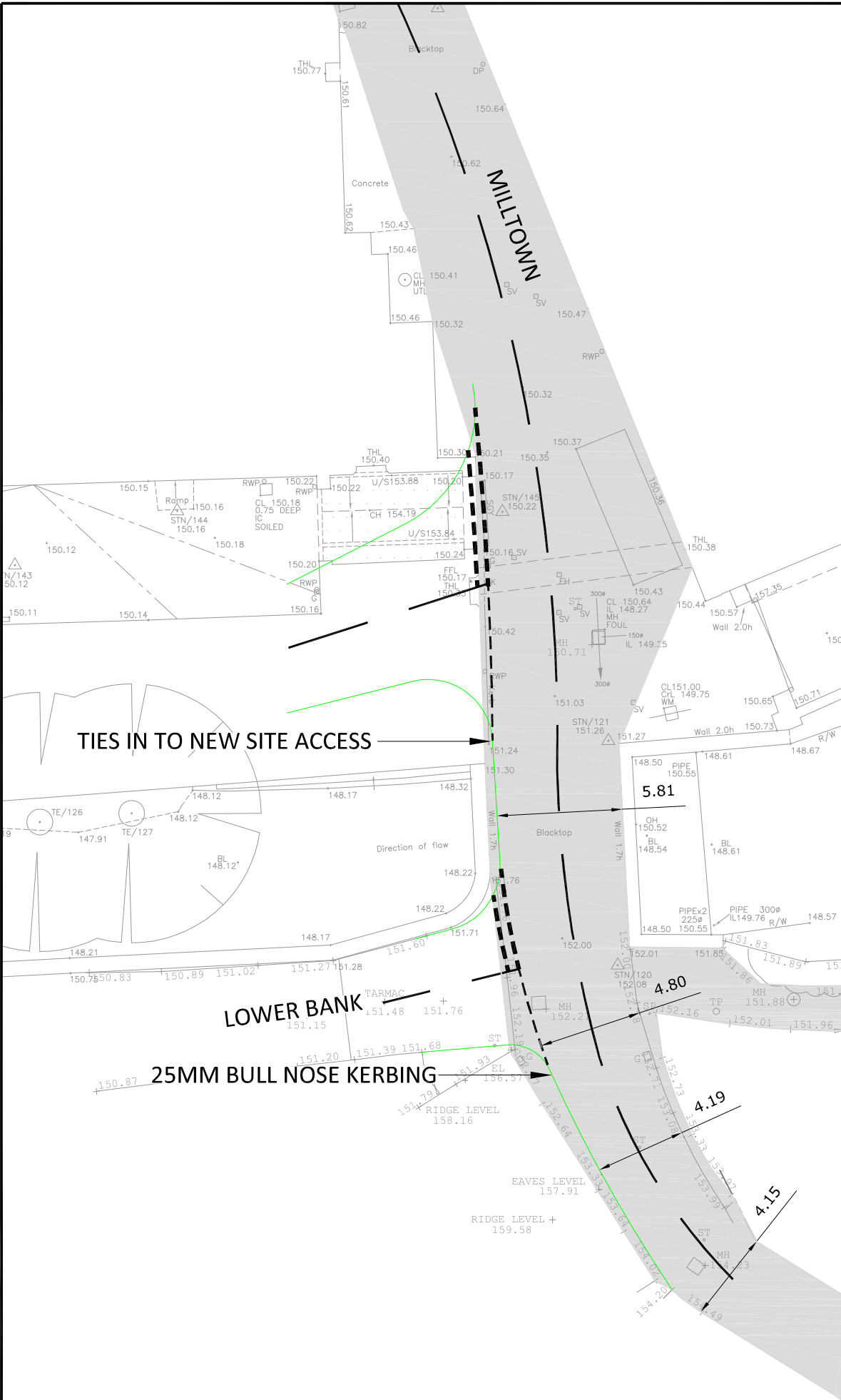
LARGE CAR TRACK @ 1:500 SCALE
