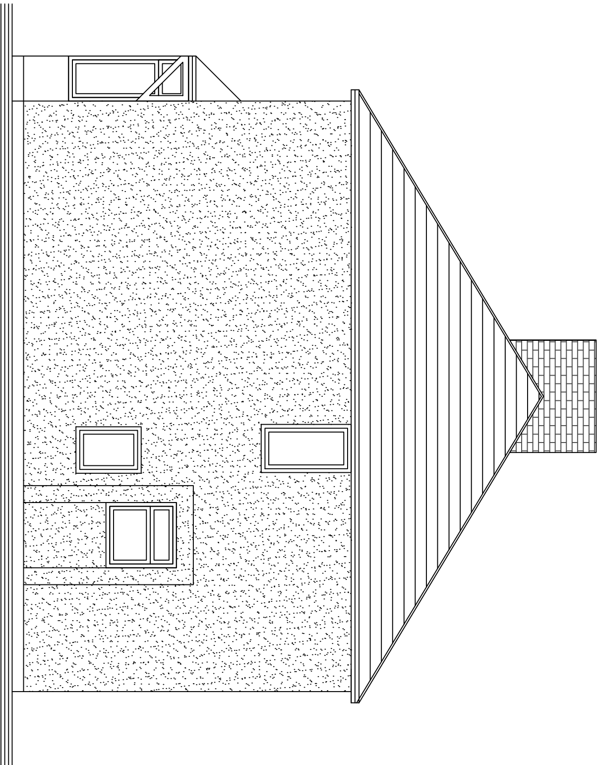
SIDE ELEVATION AS EXISTING 1:50
