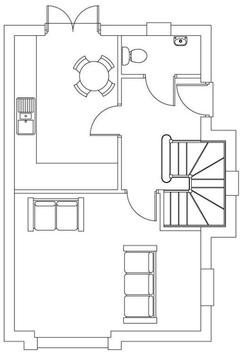
HOUSE TYPE A1 GROUND FLOOR Bed x 3 TOTAL: 944 sqft
