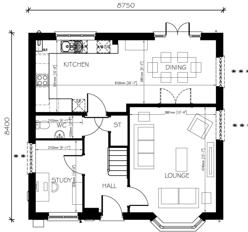
GROUND FLOOR PLAN (ALTERNATIVE LAYOUT)
