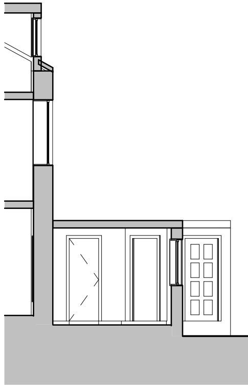
4 Courtyard 1 : 100
