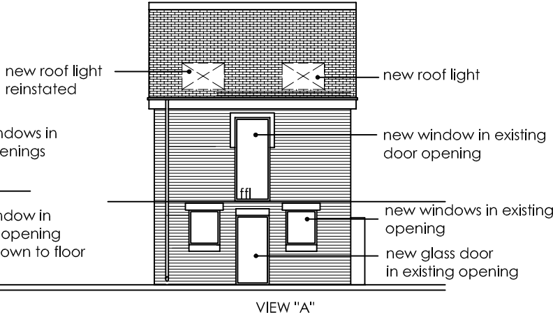
South Elevation
