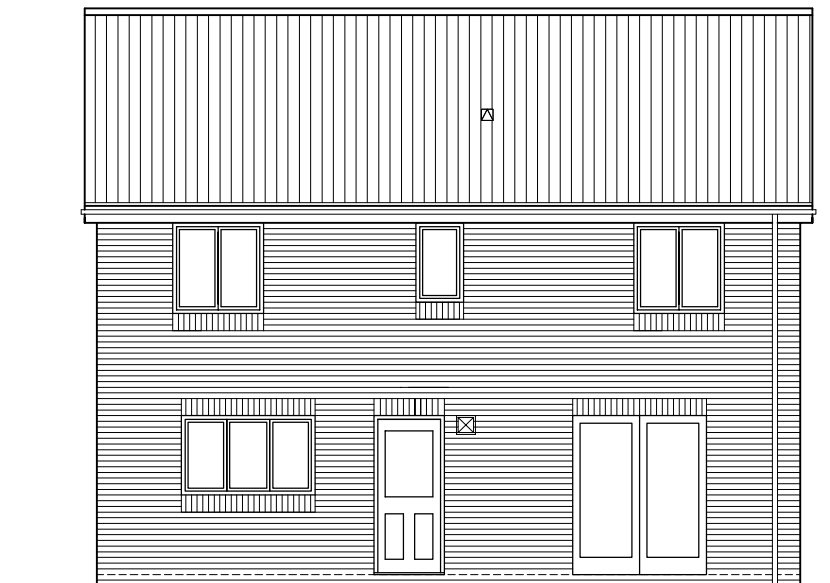
REAR ELEVATION
