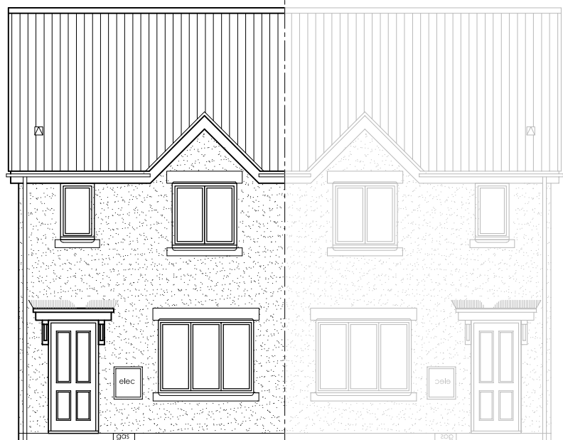
FRONT ELEVATION
