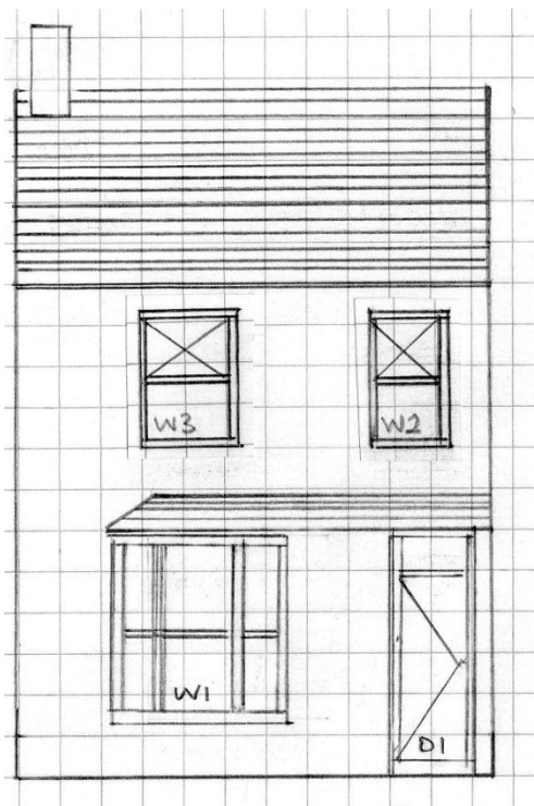
FRONT ELEVATION – South
