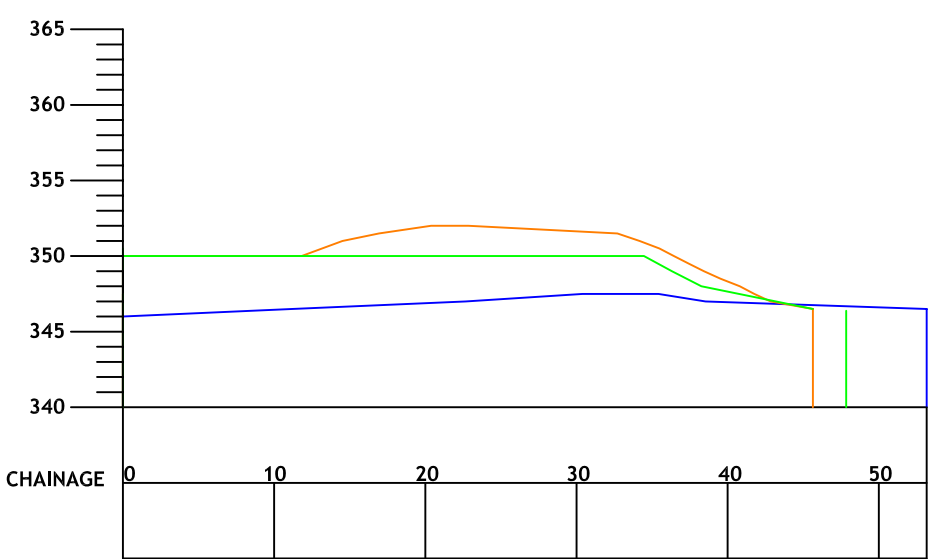
Section H-H
