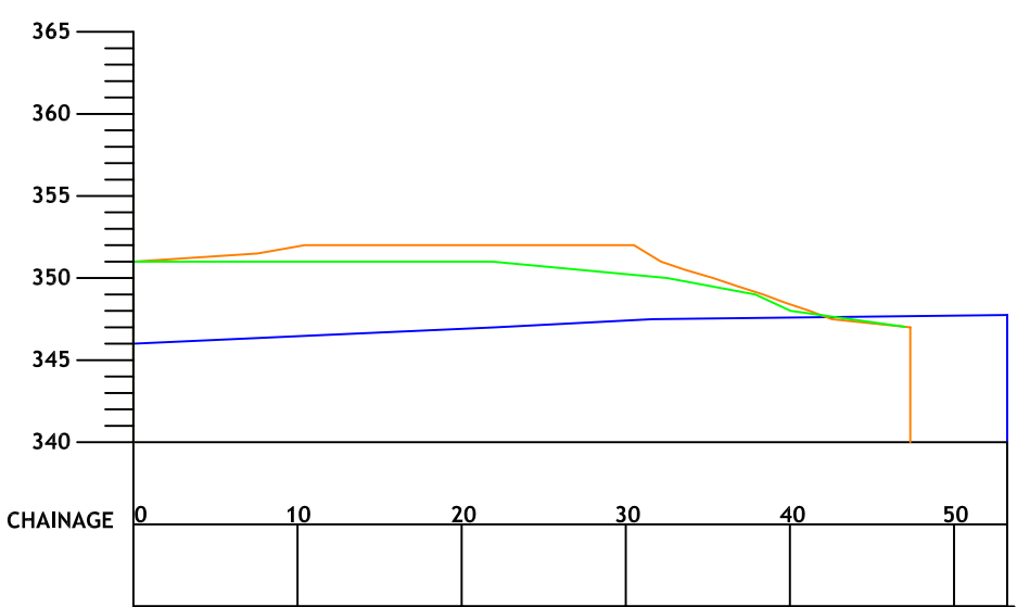
Section G-G
