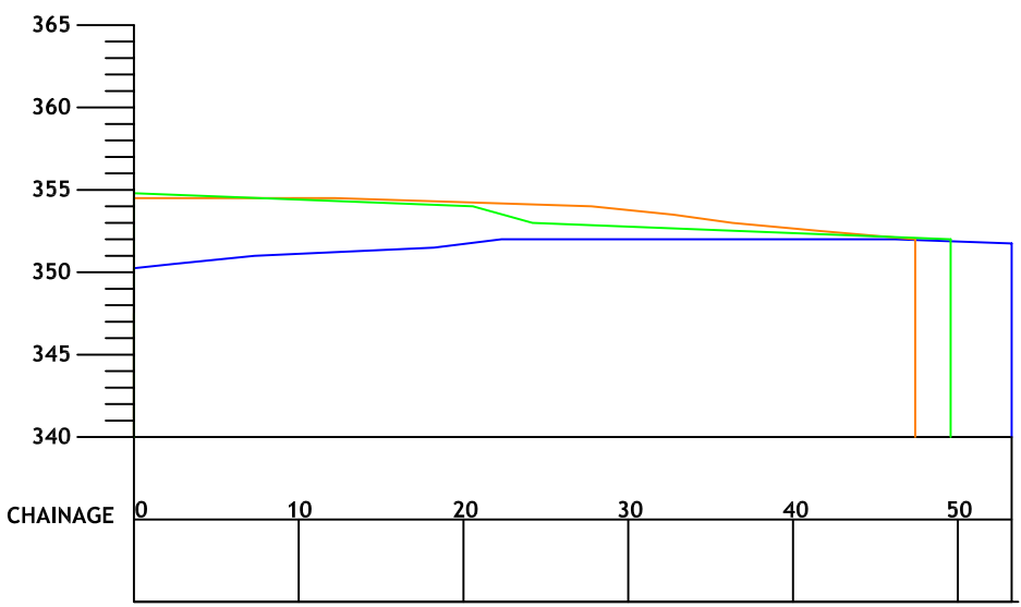
Section E-E
