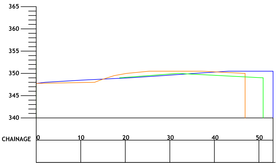
Section I-I
