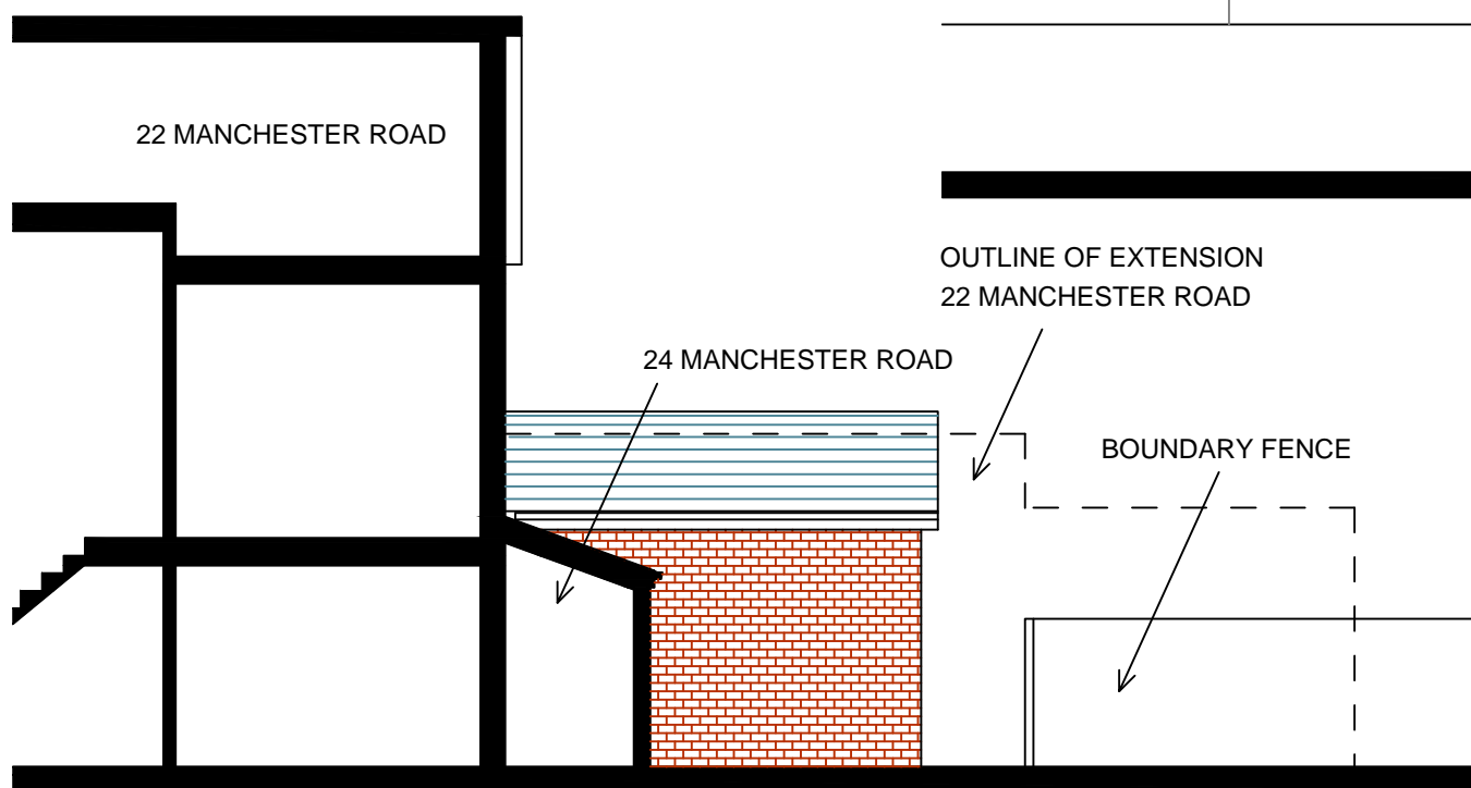
Proposed East Gable Elevations (A-A)
