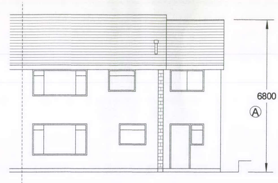
REAR ELEVATION
