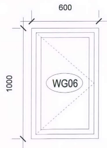
WG06 Type - Side hung flush mounted casement window Material - Idigbo hardwood solid wood Finish - Stained/oiled natural wood finish
