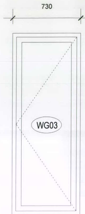
WG03 Type - Side hung flush mounted casement window Material - Idigbo hardwood frame wood Finish - Stained/oiled natural wood finish
