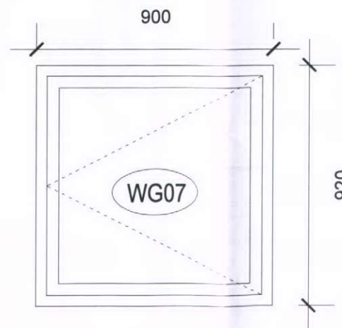
WG07 Type - Side hung flush mounted casement window Material - Idigbo hardwood solid wood Finish - Stained/oiled natural wood finish
