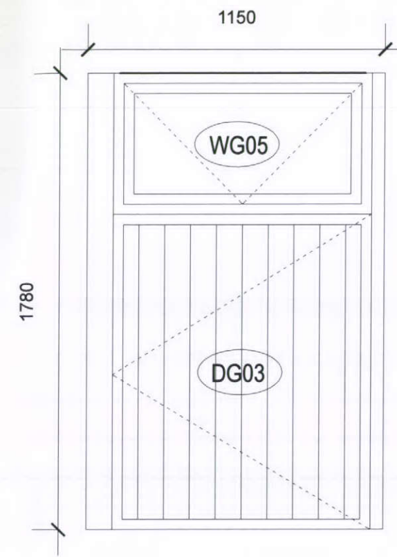
WG05 Type - Top hung flush mounted casement window Material - Idigbo hardwood frame wood Finish - Stained/oiled natural wood finish
