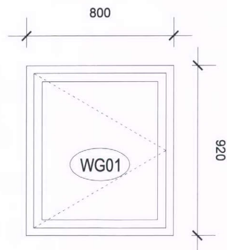
WG01 Type - Side hung flush mounted casement window Material - Idigbo hardwood frame wood Finish - Stained/oiled natural wood finish
