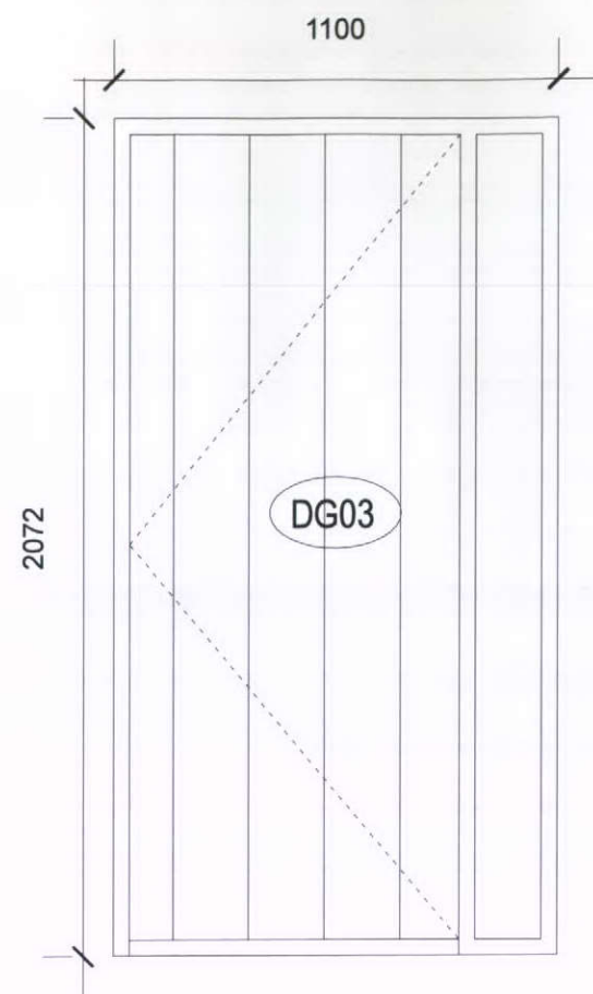
DG03 Type - Inward opening entrance door with side glazed panel Material - Idigbo hardwood solid wood Finish - Stained/oiled natural wood finish
