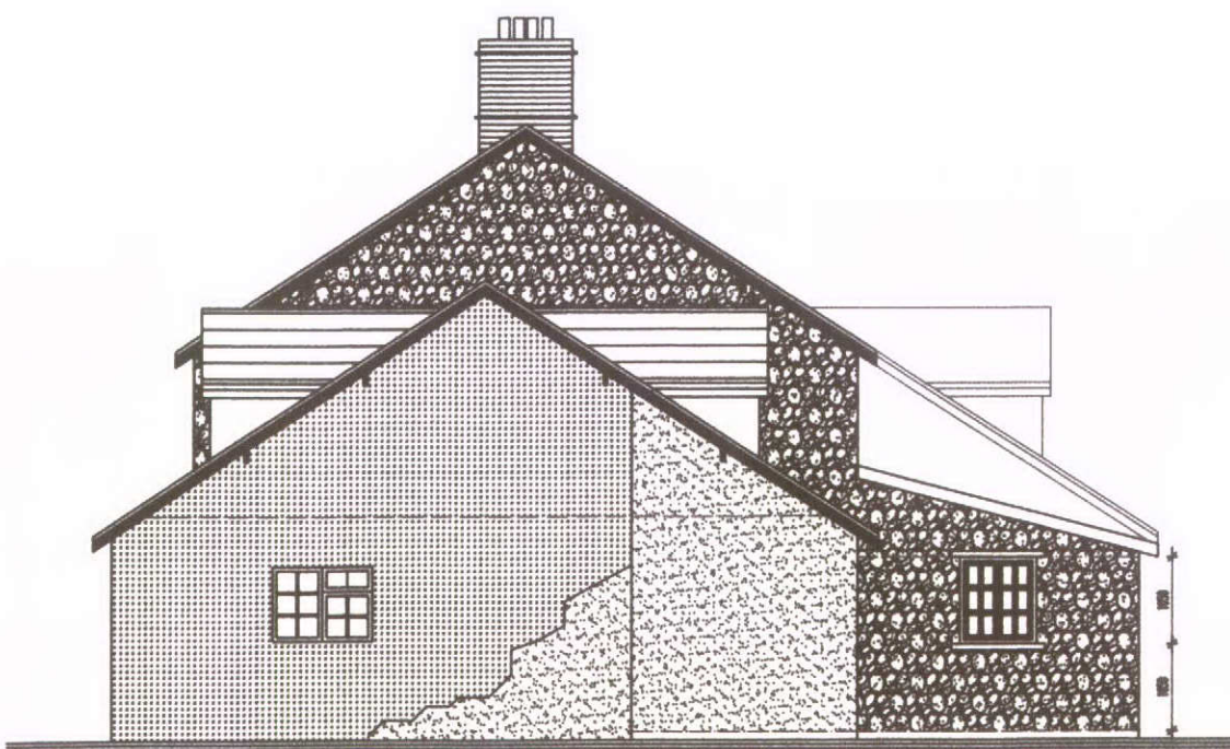
SIDE ELEVATION TO no.41
