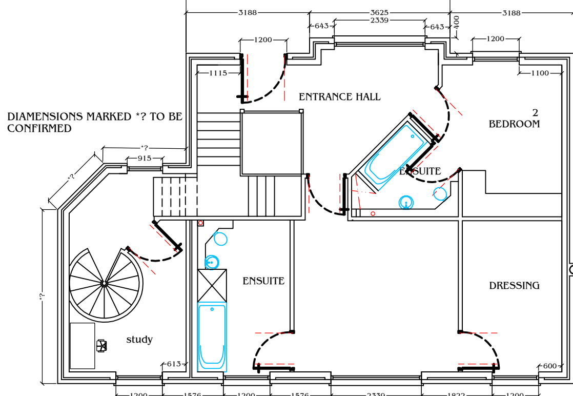
EXISTING APPROVED UPPER GROUND FLOOR PLAN 1:100
