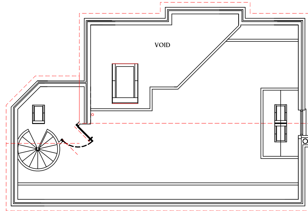
EXISTING APPROVED LOFT FLOOR PLAN 1:100
